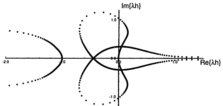
6th order Adams-Bashforth-Moulton
