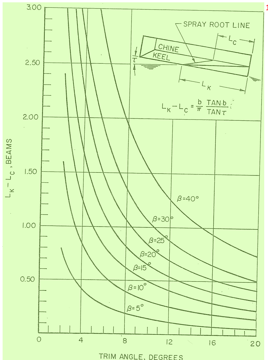
Fig. 6 L_k - L_c versus trim and deadrise
