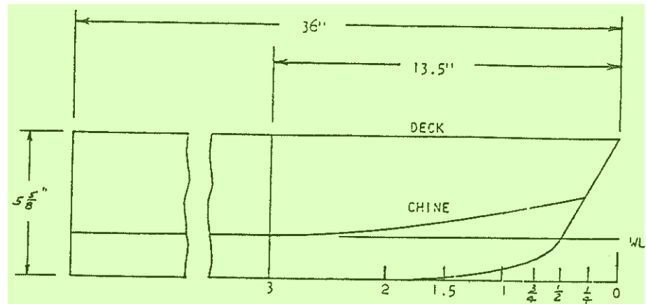
Fig. 16 Lines of prismatic model with conventional bow 4
