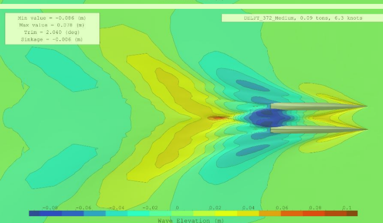
Figure 10: Free surface evolution (same scale) from 5.3 to 7.9 knots 2
