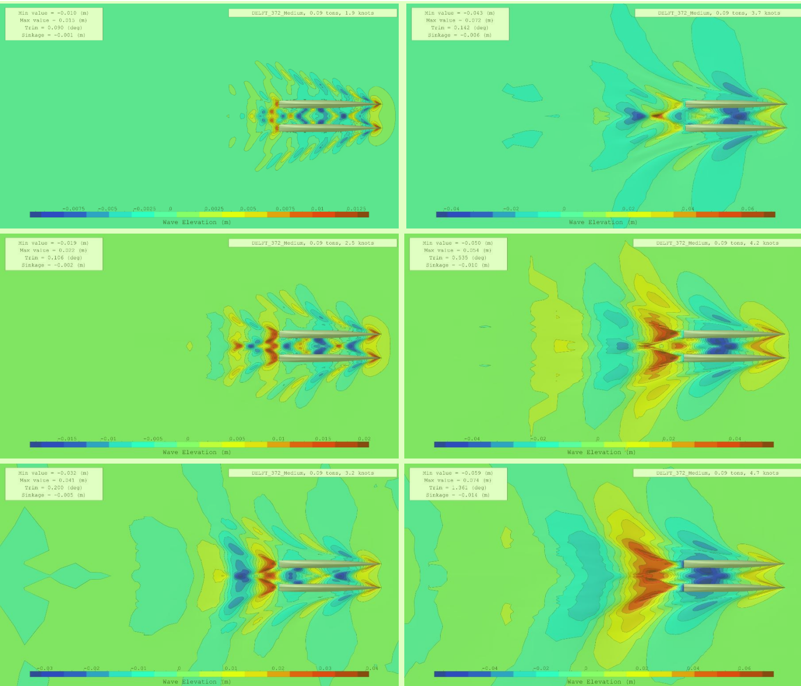
Figure 11: Free surface evolution (independent scale) from 1.9 to 4.7 knots 3
