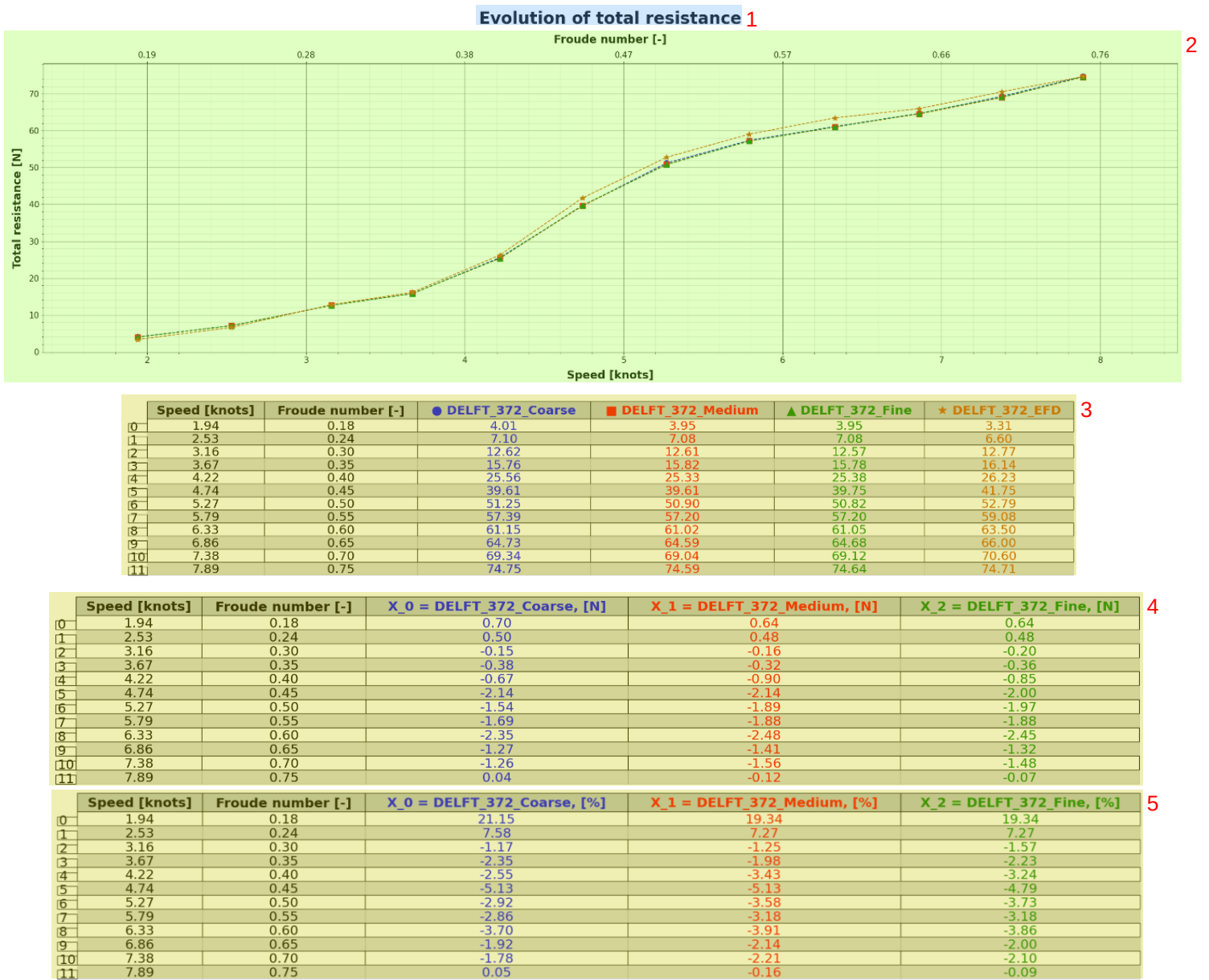
Figure 5: Evolution (up), difference [N] (middle) and difference [%] (bottom) of total resistance 6
