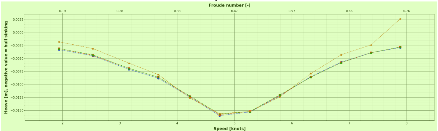
Evolution of dynamic heave attitude 6
