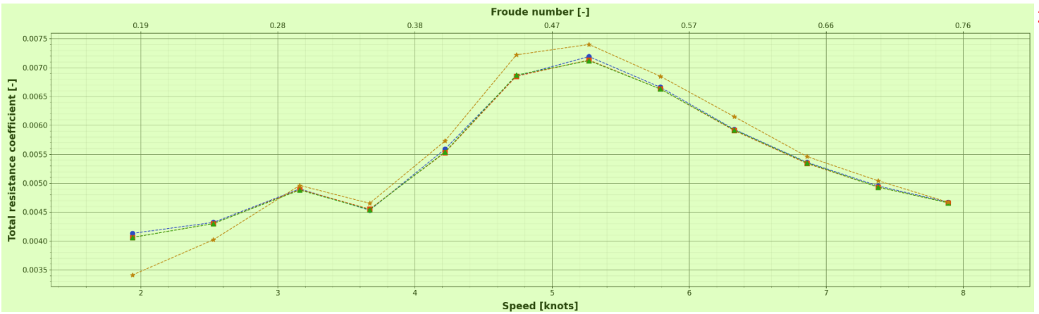
Evolution of total resistance coefficient 1
