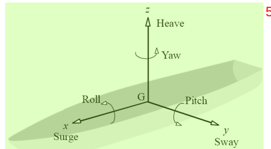
Figure 2: Sign convention illustration 6
