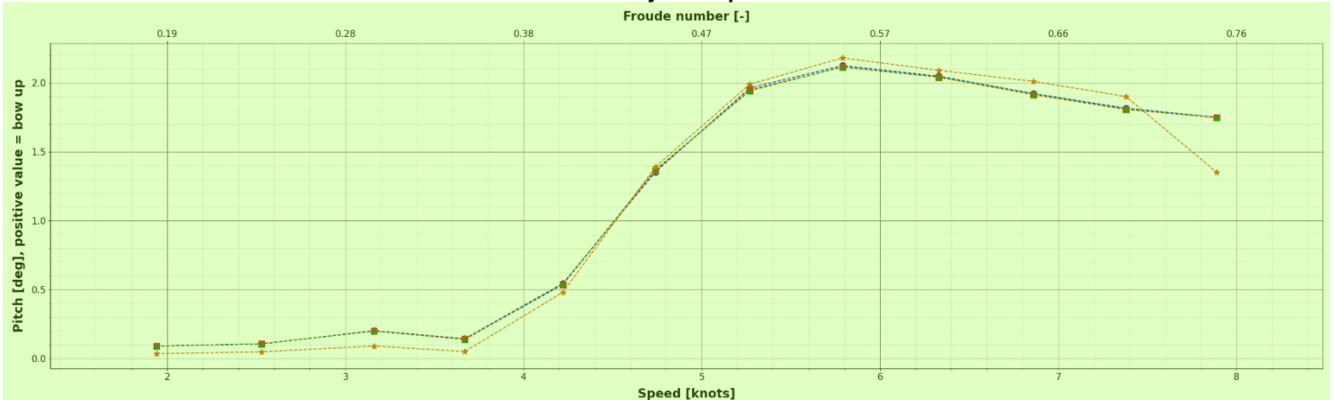
Evolution of dynamic pitch attitude 7
