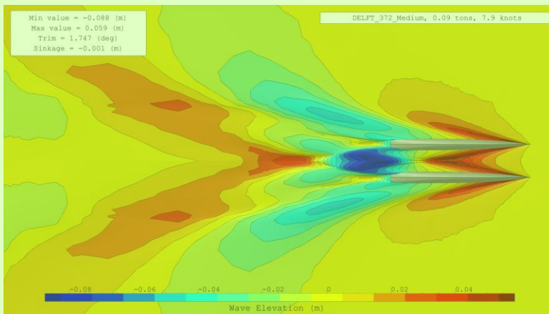
Figure 12: Free surface evolution (independent scale) from 5.3 to 7.9 knots 2
