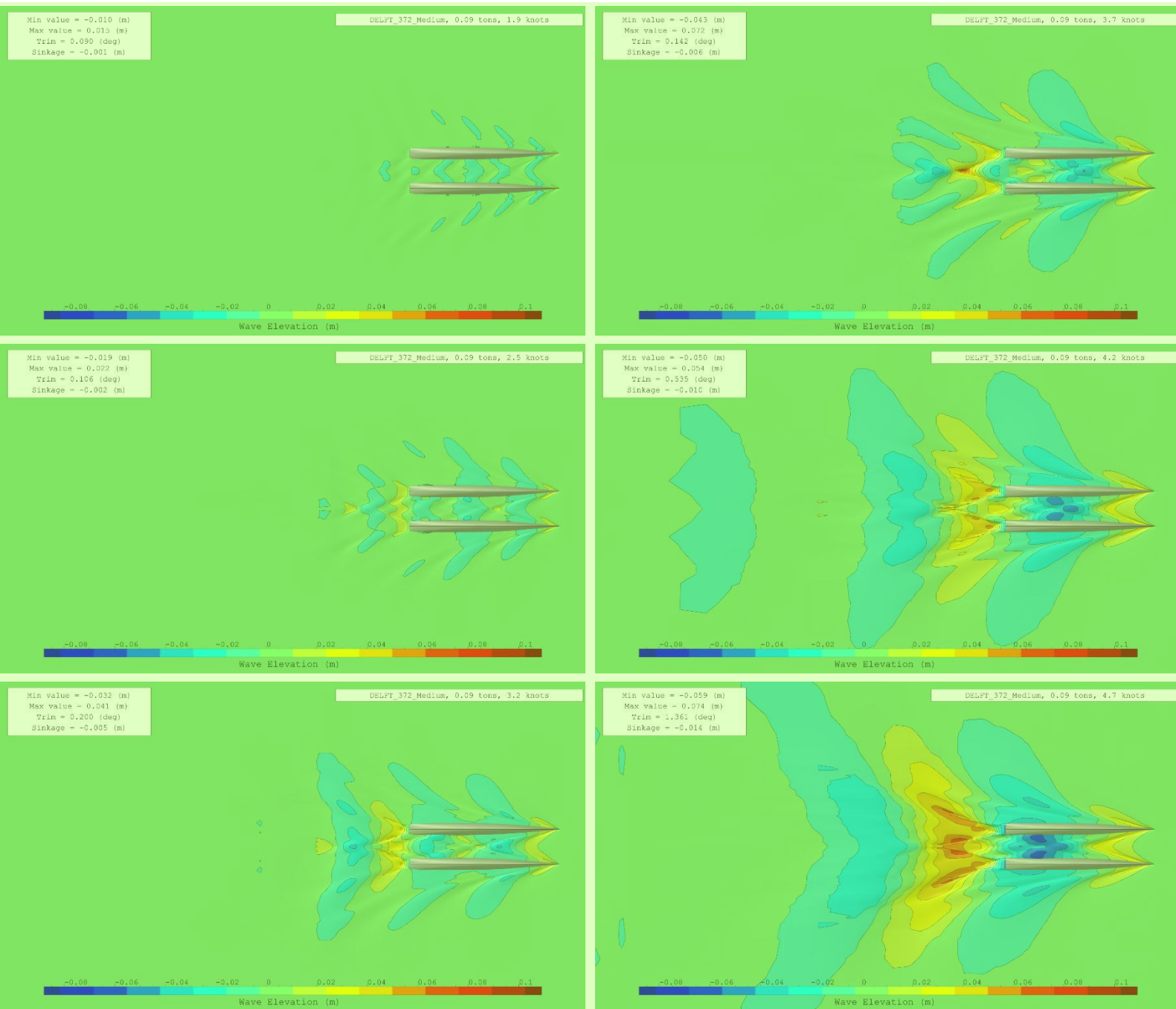
Figure 9: Free surface evolution (same scale) from 1.9 to 4.7 knots 4
