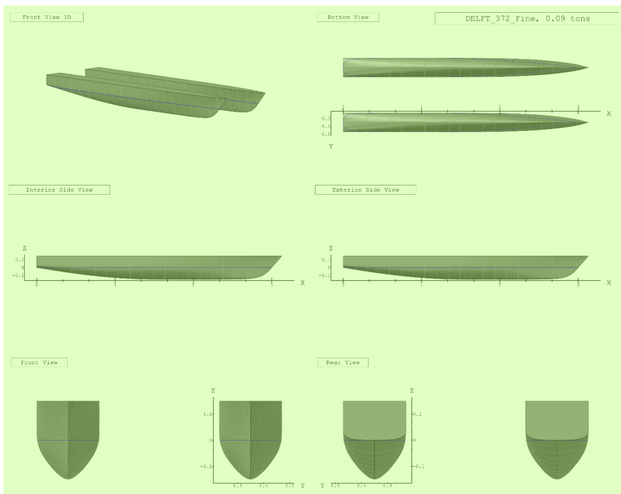
Figure 1: DELFT 372 CAD model 6
