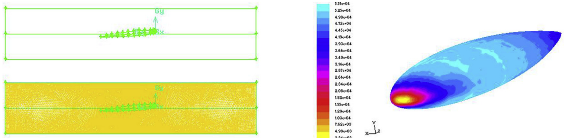
Fig. 7. Calculation of lift force of SSB by CFD. (a) SSB and fluid domain numerical setup. (b) Pressure distribution on the advancing SSB.
