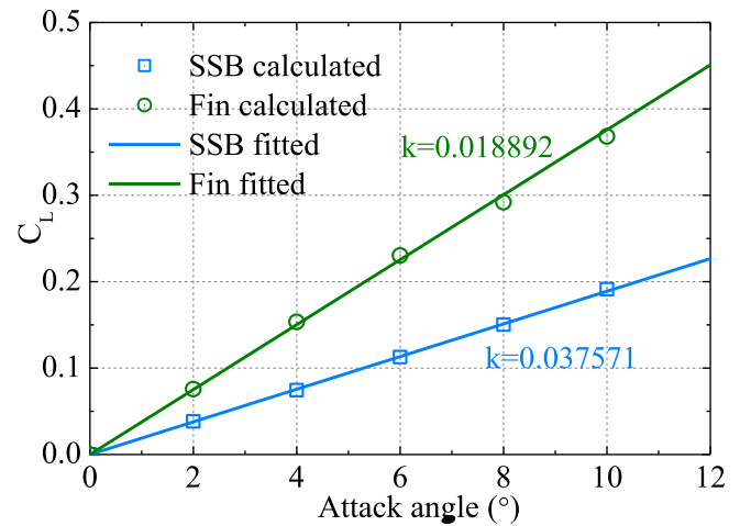
Fig. 8. Lift coefficients of SSB and fin.
