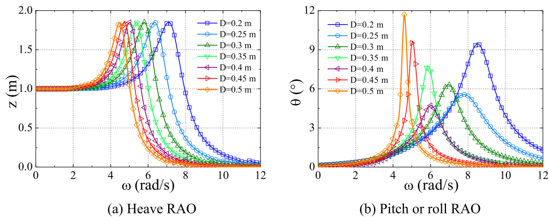
Fig. 22. Motion response transfer function of buoy at different diameter.
