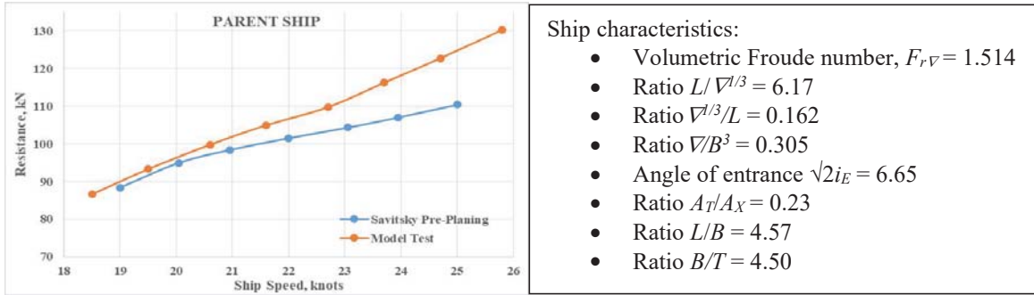
FIGURE 5. Comparison of the resistance for the parent ship
