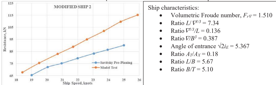
FIGURE 7. Comparison of the resistance for the modified ship 2
