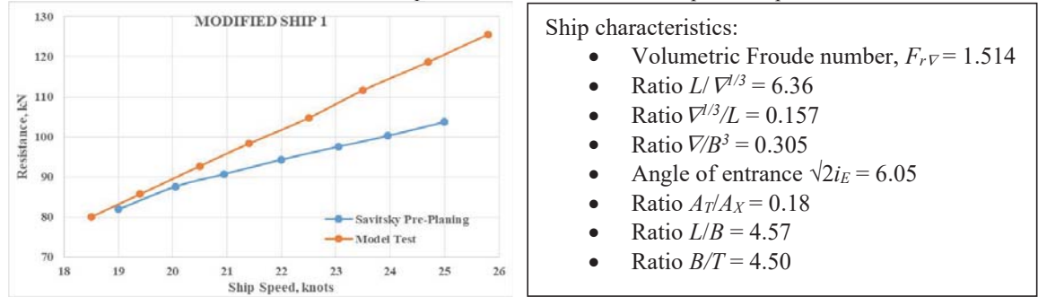
FIGURE 6. Comparison of the resistance for the modified ship 1
