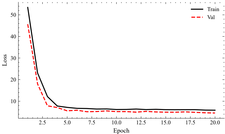
B2-GPU96 NATL60 crop96 (20 ep) - not paper Table
