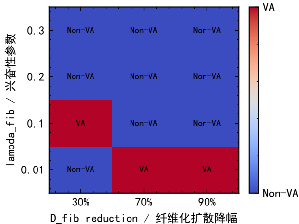
诱发性相图 Inducibility (annulus)
