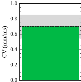
2D CV
