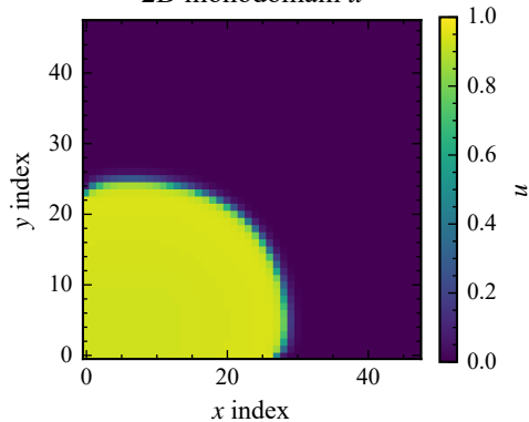
2D monodomain u
