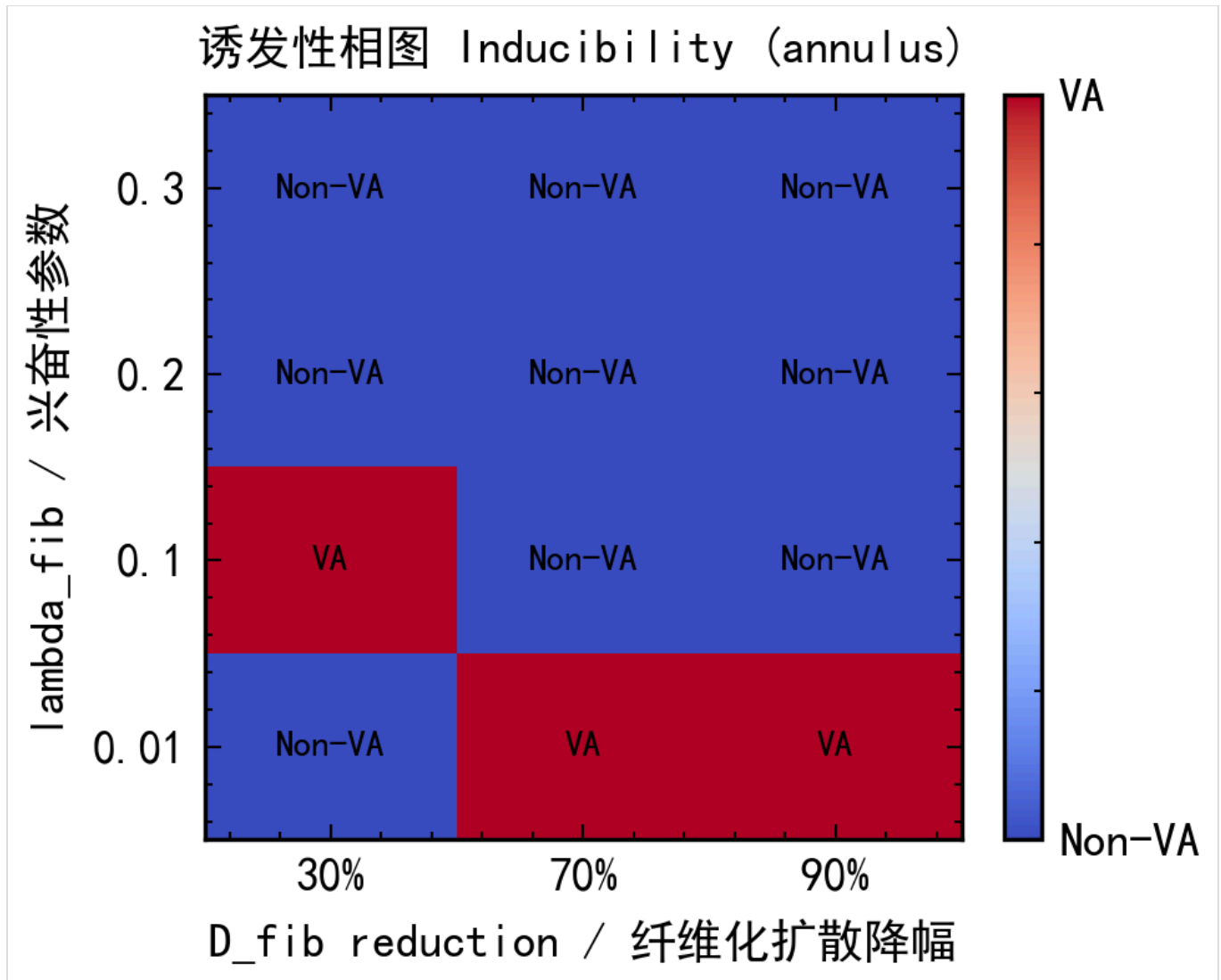
图3. 钉扎环 \lambda_{\text{fib}} \times D_{\text{fib}} 诱发性相图
