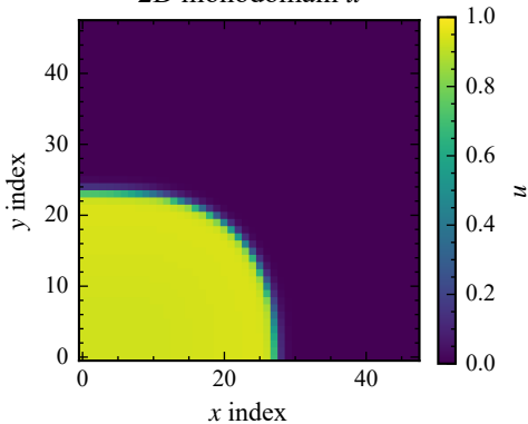
2D monodomain u
