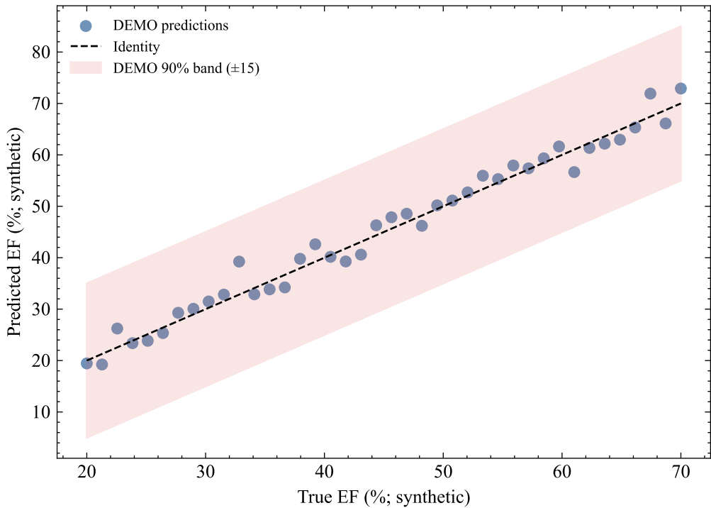
Split-conformal interval cartoon — DEMO
