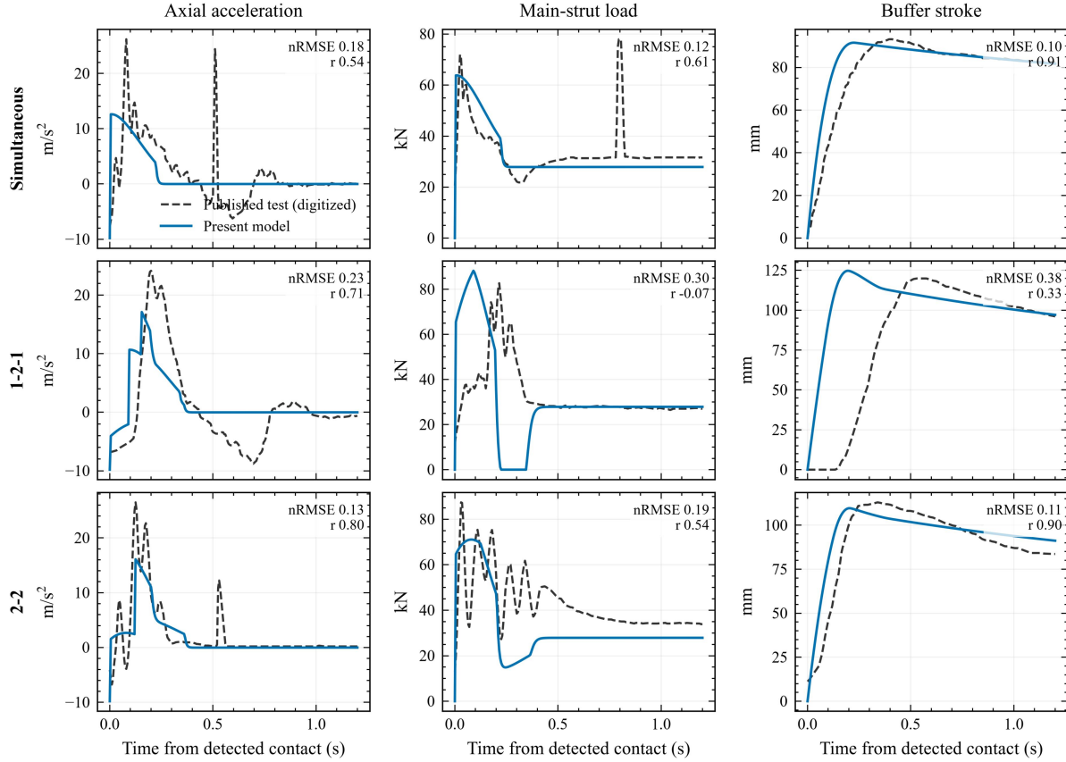
Figure 4. Comparison of the present reduced model with Yang et al. (2026). Grey dashed curves are digitized experimental data; blue solid curves are present calculations. Model parameters were fitted only to simultaneous touchdown.
