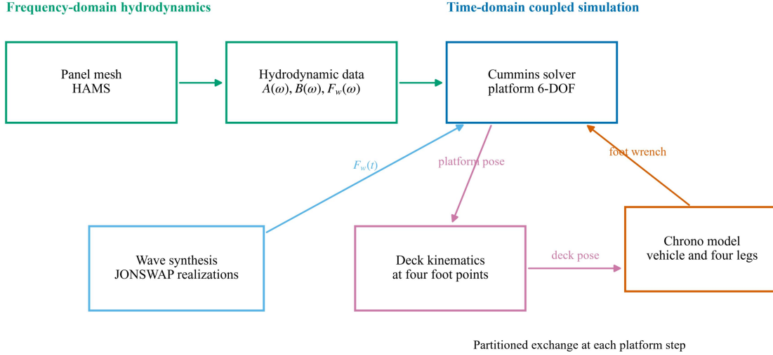
Figure 1. Numerical arrangement of the proposed framework. HAMS is used without changes to its source code. The time-domain, deck-point and multibody calculations are external modules.
