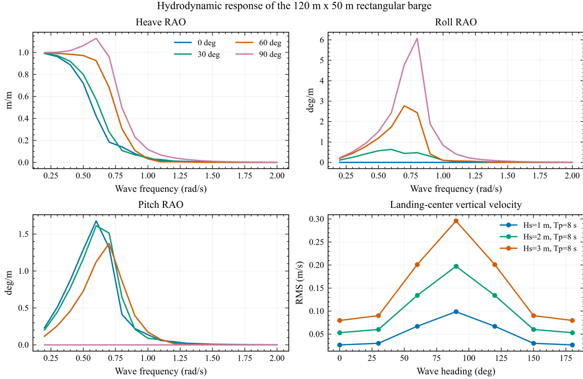
Figure 5. Landing-center HAMS RAOs and JONSWAP vertical-velocity RMS. All curves are calculated with the locally compiled HAMS executable and the parameterized mesh in Figure 2.
