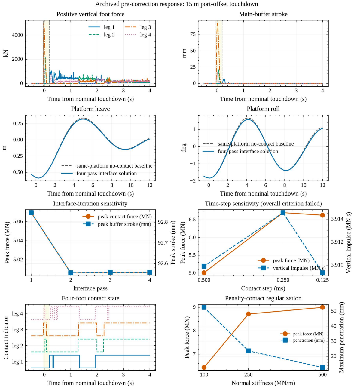
Figure 6. Archived pre-correction four-foot calculation, retained for numerical diagnosis. The yellow interval marks first-to-last initial contact, and production curves use a nominal 0.5 ms contact step. Force and impulse are positive world-vertical quantities, not deck-normal projections. Main traces use four passes over 506-526 s; step and stiffness studies use two and one passes, respectively, over 506-516 s. All panels retain pre-correction values; corrected coupled results remain pending.
