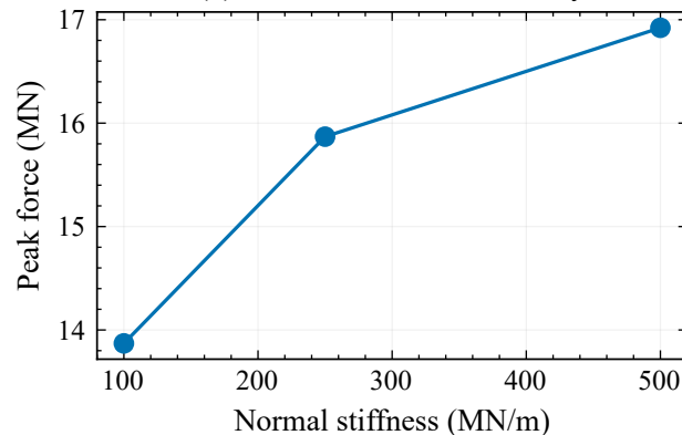
(h) Contact-stiffness sensitivity
