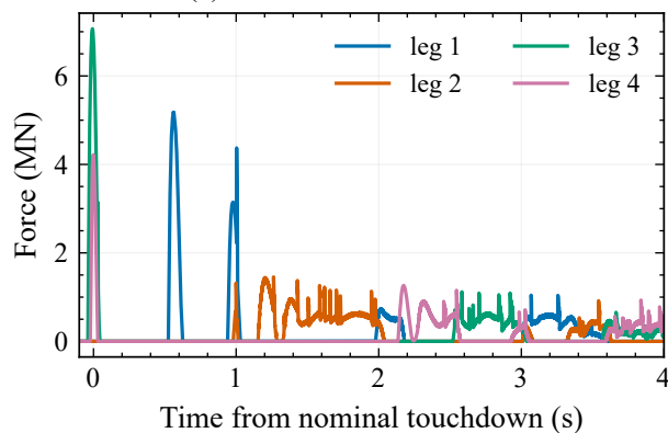
(c) Platform response
