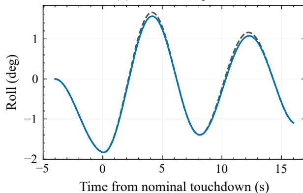
(f) Contact-step sensitivity
