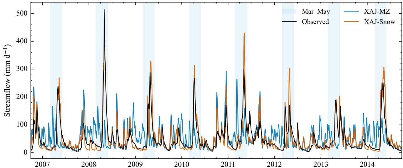
camels_01013500 test hydrograph (XAJ-MZ vs XAJ-Snow)
