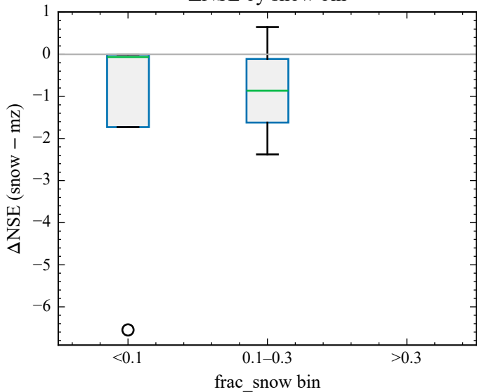
\Delta NSE by snow bin
