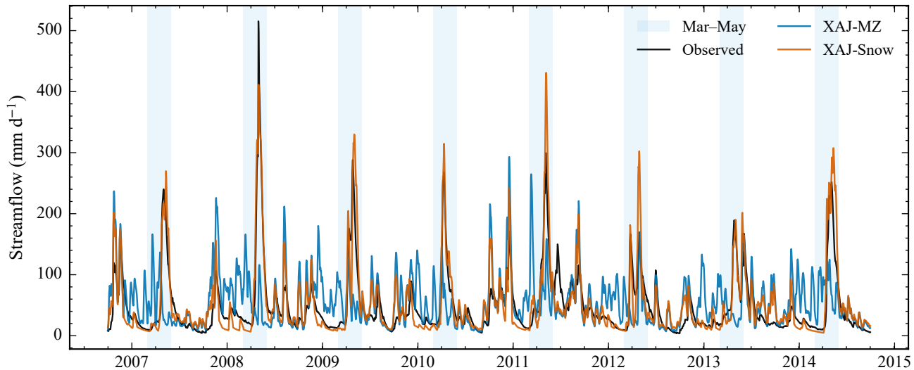
camels_01013500 medium: Observed / XAJ-MZ / XAJ-Snow
