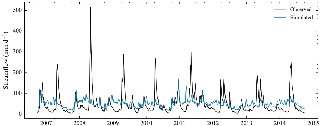
camels_01013500 XAJ-MZ (historical scipy) (rep=v2 refine)
