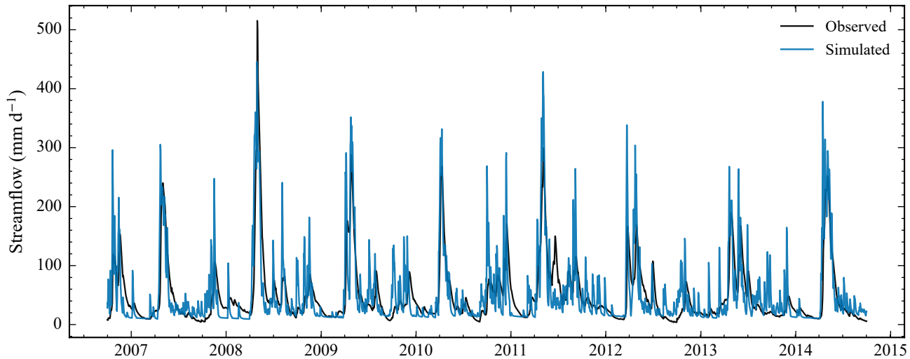
camels_01013500 XAJ-Snow smoke (rep=120)
