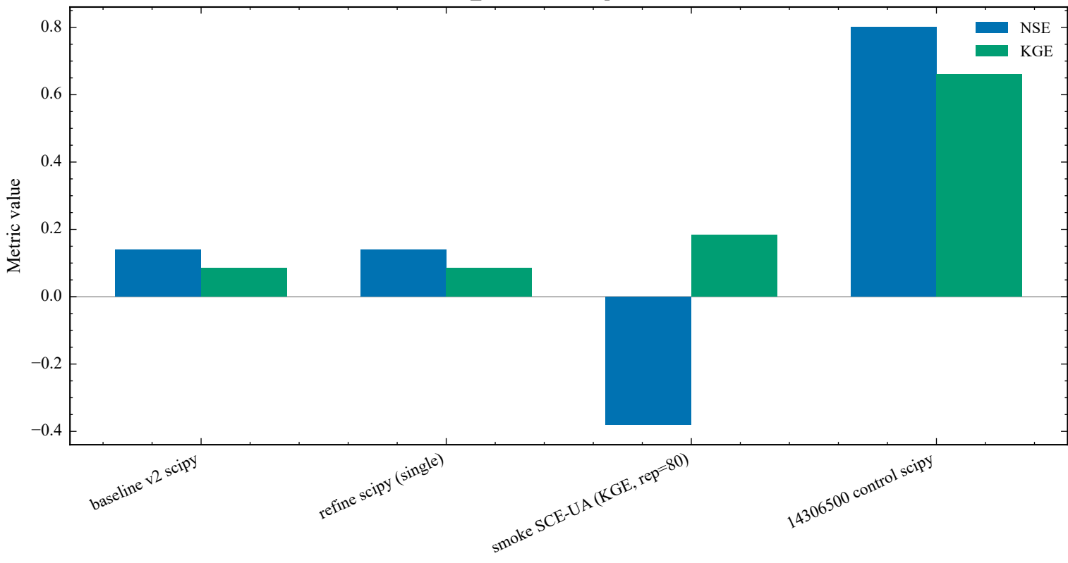
camels_01013500 test-period metrics
