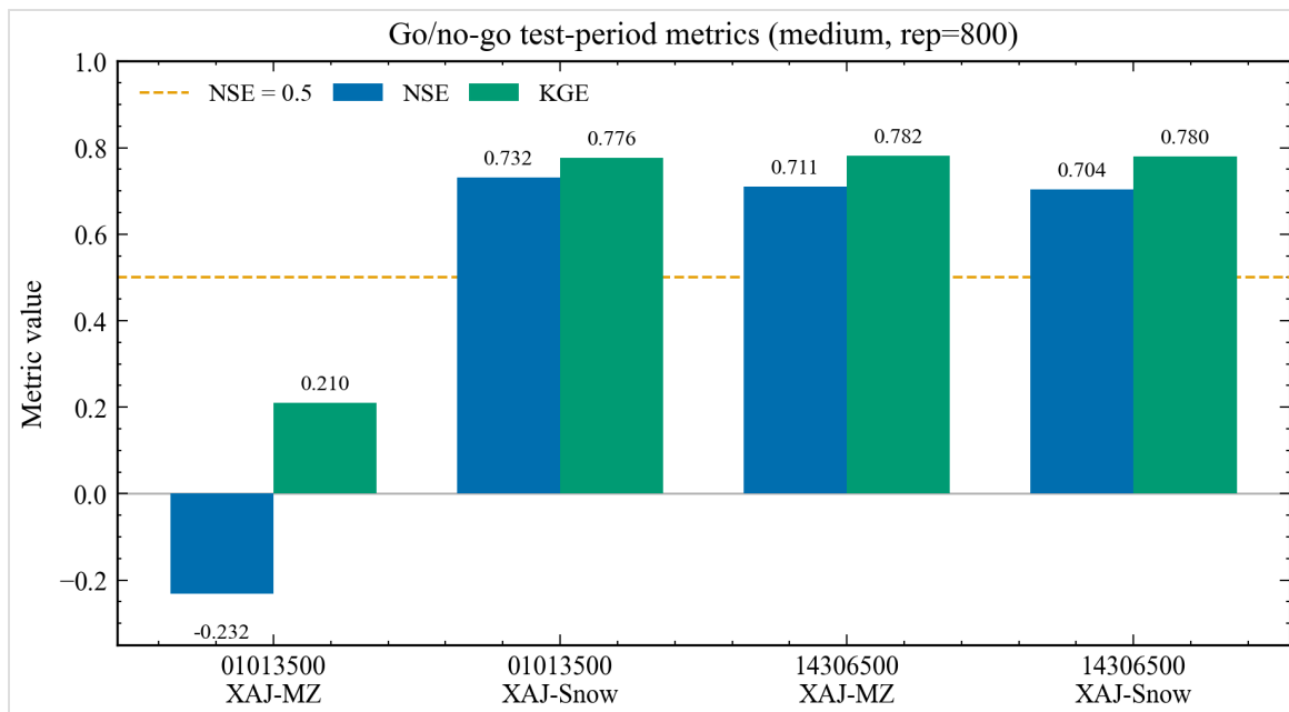
图 1. Go/no-go 成对样本外 NSE 与 KGE 柱状对比. Data source: basins_metrics.csv under results/xaj_snow_go_nogo/*/evaluation_test/.
