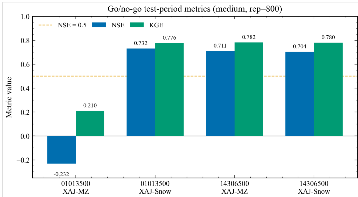
Figure 1. Paired out-of-sample NSE and KGE for the pilot basins. Data source: paired go/no-go basins_metrics.csv (SCE-UA+KGE, rep=800).
