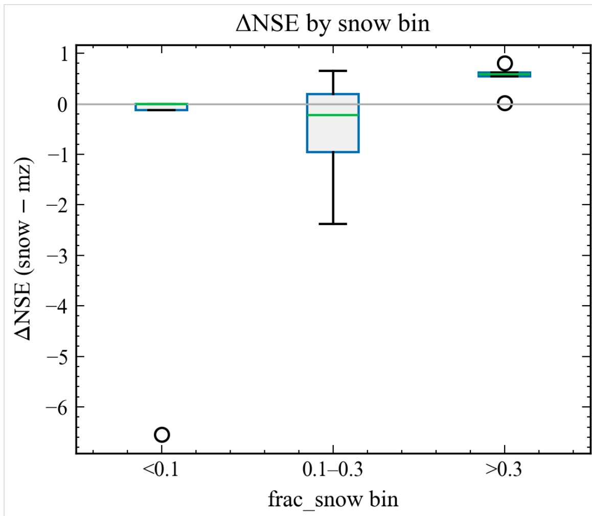
Figure 7. Screening-batch \Delta NSE by snow-fraction bin ( n=14 , \text{rep}=200 ). Data source: results/diagnostics/batch1_paired_metrics.csv.
