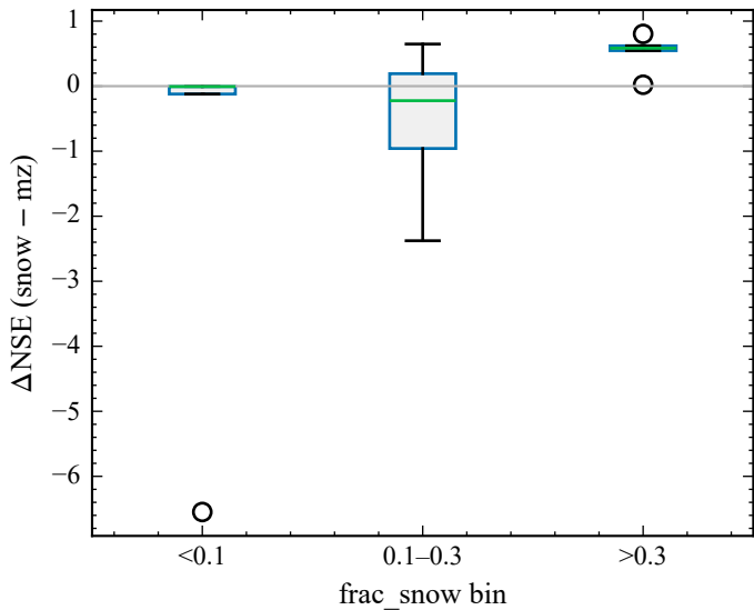
\Delta\text{NSE} by snow bin
