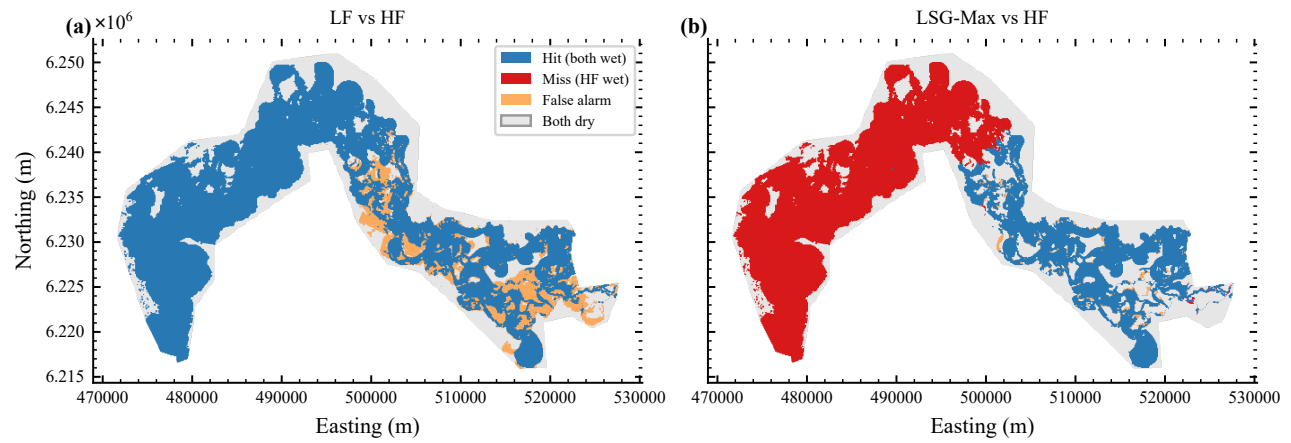
Figure 2b. Chowilla E1 extent H/M/FA maps. Supports the wet_train vs all_cells protocol anti-case.
