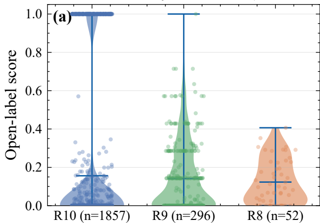
Score distribution by resolution (mean rollup)
