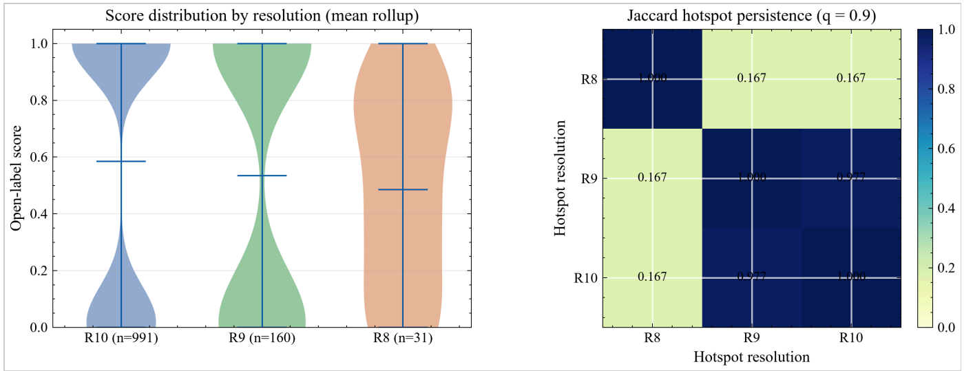
Figure 5. Resolution effects on the open-label score surface. (a) Violin plots of the score distribution at R10 ( n = 991 ), R9 ( n = 160 , mean rollup), and R8 ( n = 31 , mean rollup), showing variance compression as the grid coarsens. (b) Jaccard hotspot-persistence matrix (0.9-quantile thresholds) between hotspot sets at R10, R9, and R8, computed on the coarser support of each pair so the R10-vs-R9 and R10-vs-R8 entries reproduce the ladder in Fig. 4.
