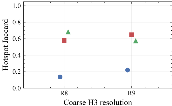
Area-weighted soft Jaccard
