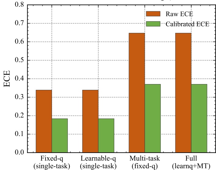
ODIR val ECE before / after T-scaling (SYNTHETIC)
