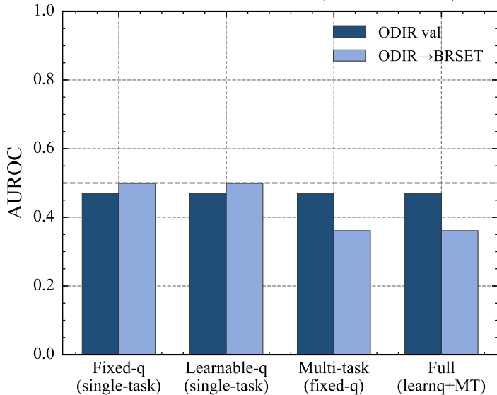
ODIR-D head AUROC (SYNTHETIC)
