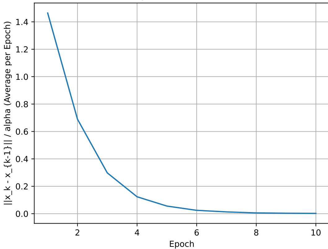
Convergence of Proximal SAGA
