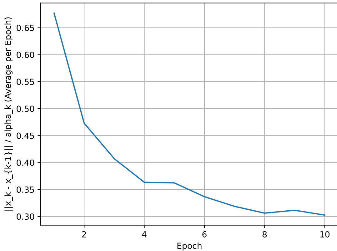
Convergence of SGD
