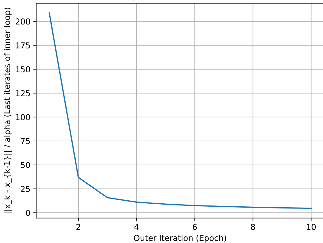
Convergence of Proximal SVRG++
