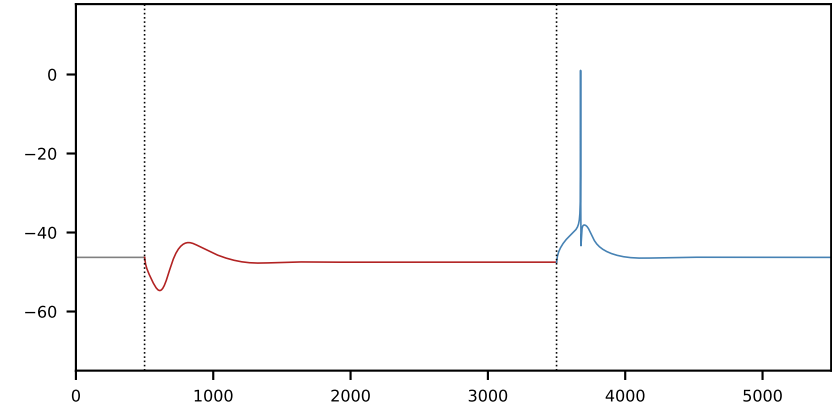
tonic firing, then a sustained (tonic) rebound held=-2.94 nA, injected=-1.46 nA
