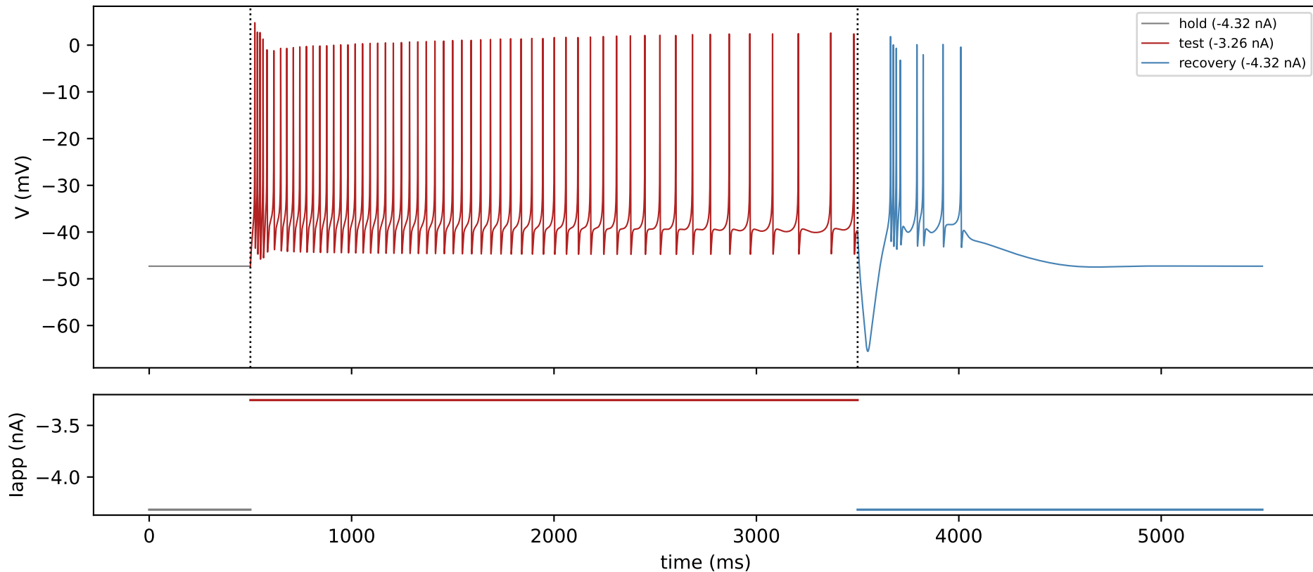
XB2IQX — held=-4.32 nA, injected=-3.26 nA — test: tonic, rebound: bursting_rebound
