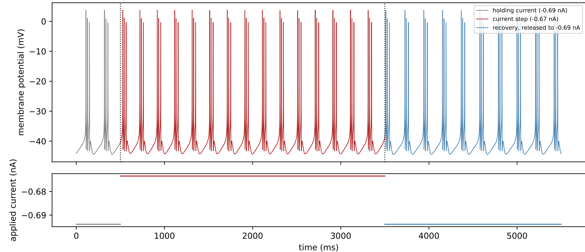
DFJ1K3: bursting during the current step, then a burst-like rebound
