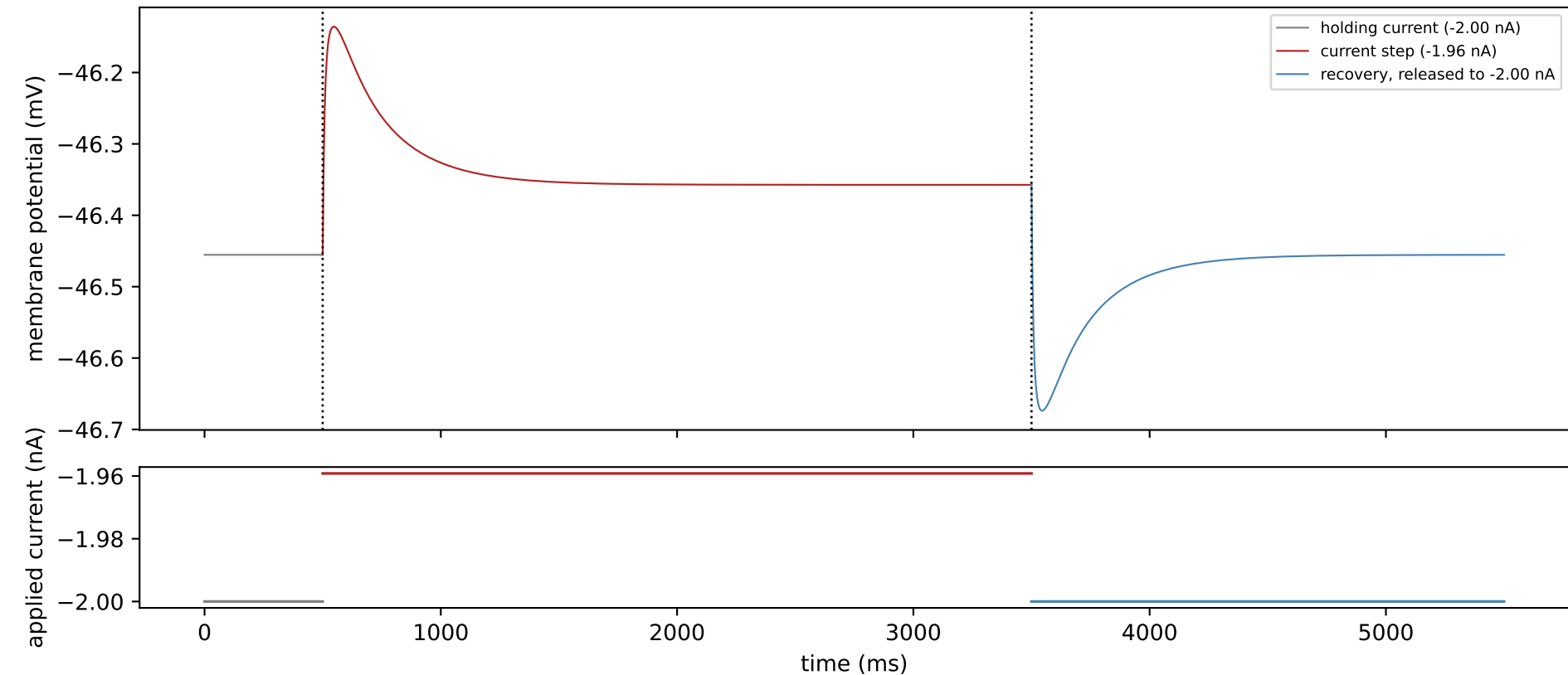
DFJ1K3: silent (no firing) during the current step, then no rebound
