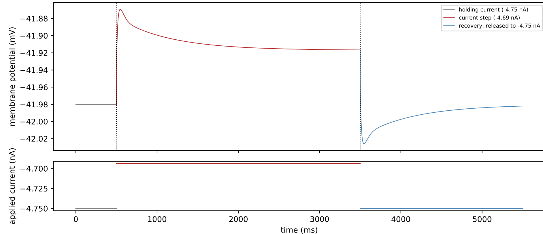
MXIC4S: silent (no firing) during the current step, then no rebound
