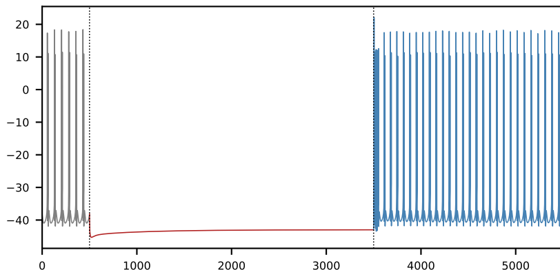
silent (no firing), then a burst-like rebound held=-0.48 nA, injected=-5.75 nA
