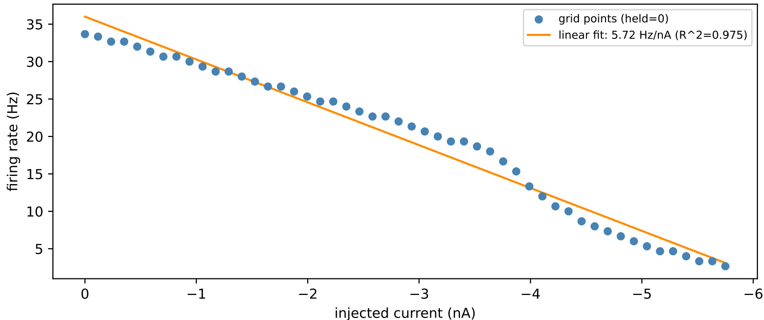
MXIC4S -- firing rate vs. injected current, no holding current
