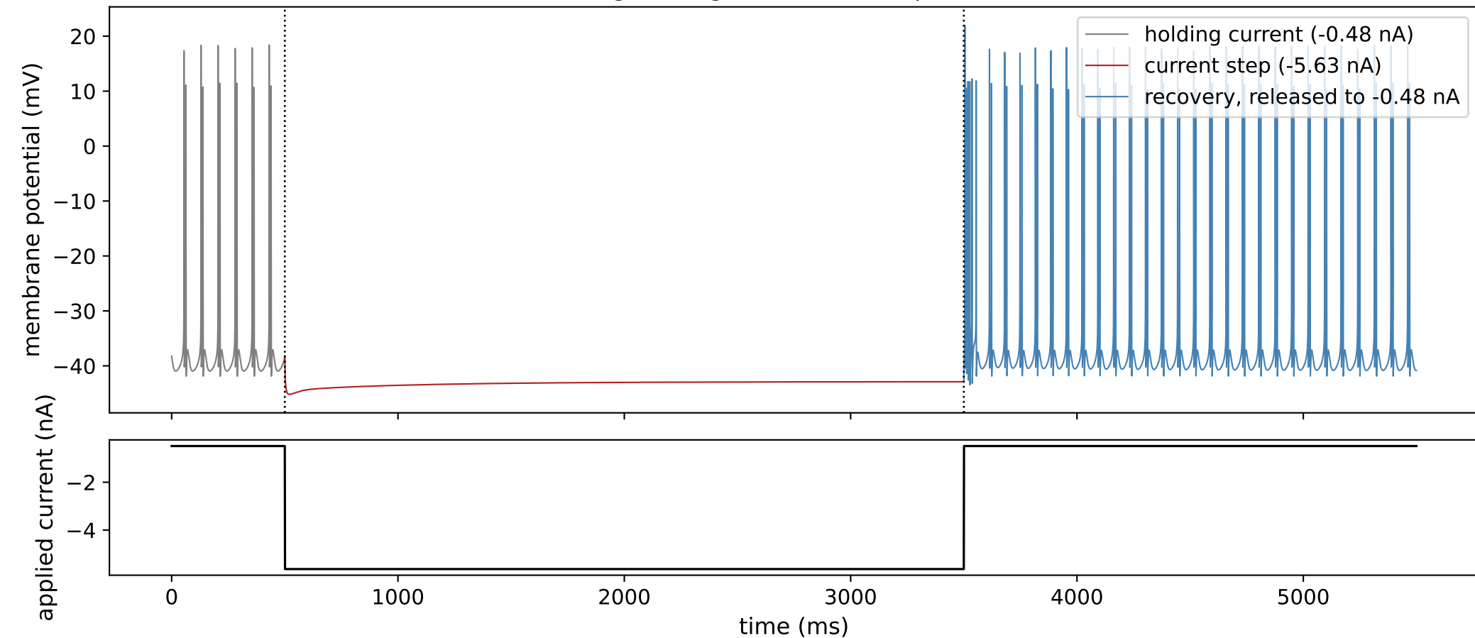
MXIC4S: silent (no firing) during the current step, then a burst-like rebound
