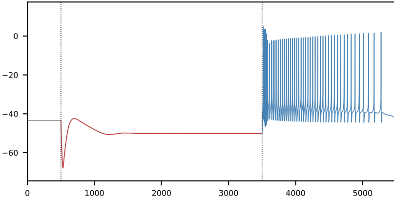
silent (no firing), then a sustained (tonic) rebound held=-2.02 nA, injected=-5.39 nA
