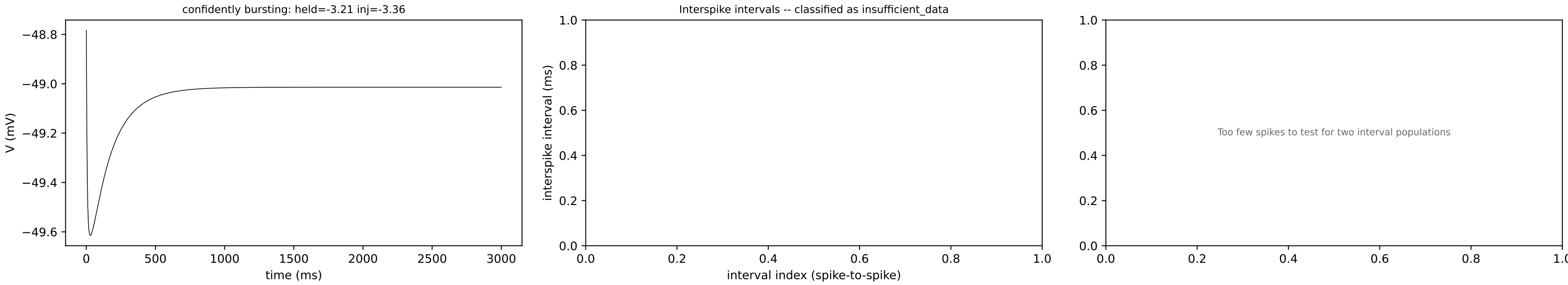
Simulated DFJ1K3 trace. This window had 0 spike(s), giving 0 interspike interval(s) -- fewer than the 6 needed to statistically test whether intervals fall into two separate populations (short, within-burst gaps vs. long, between-burst gaps), so the window defaults to 'insufficient_data'.
