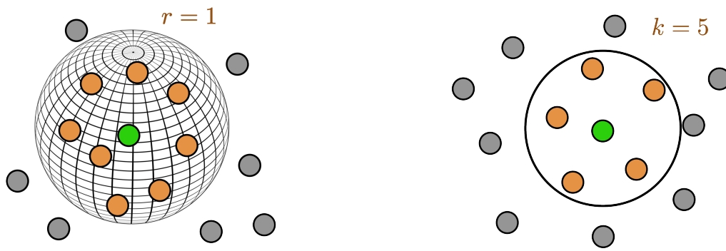
Figure 3: Spherical neighborhood (left) and KNN (right)
