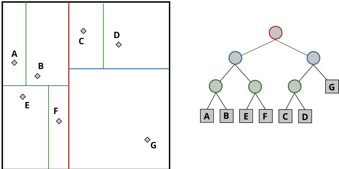
Figure 5: A kd-tree in 2-dimensional space
