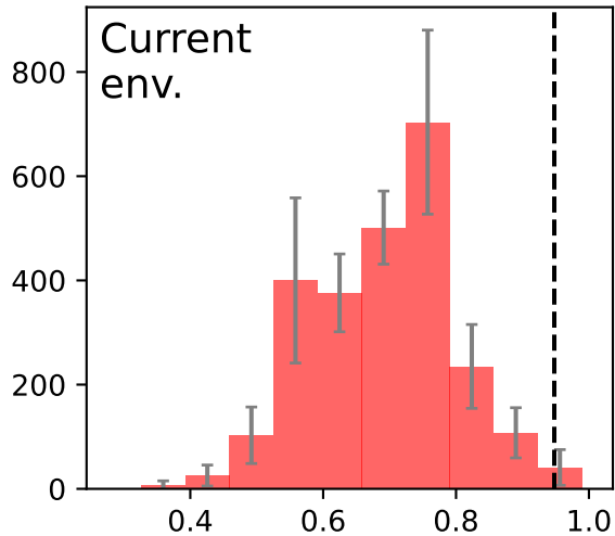
Rule 54
