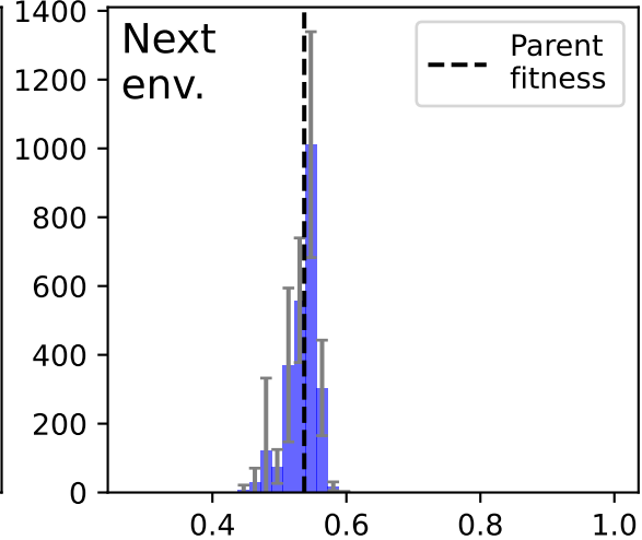
Rule 122
