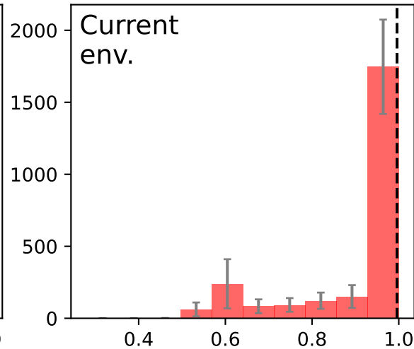
Rule 122
