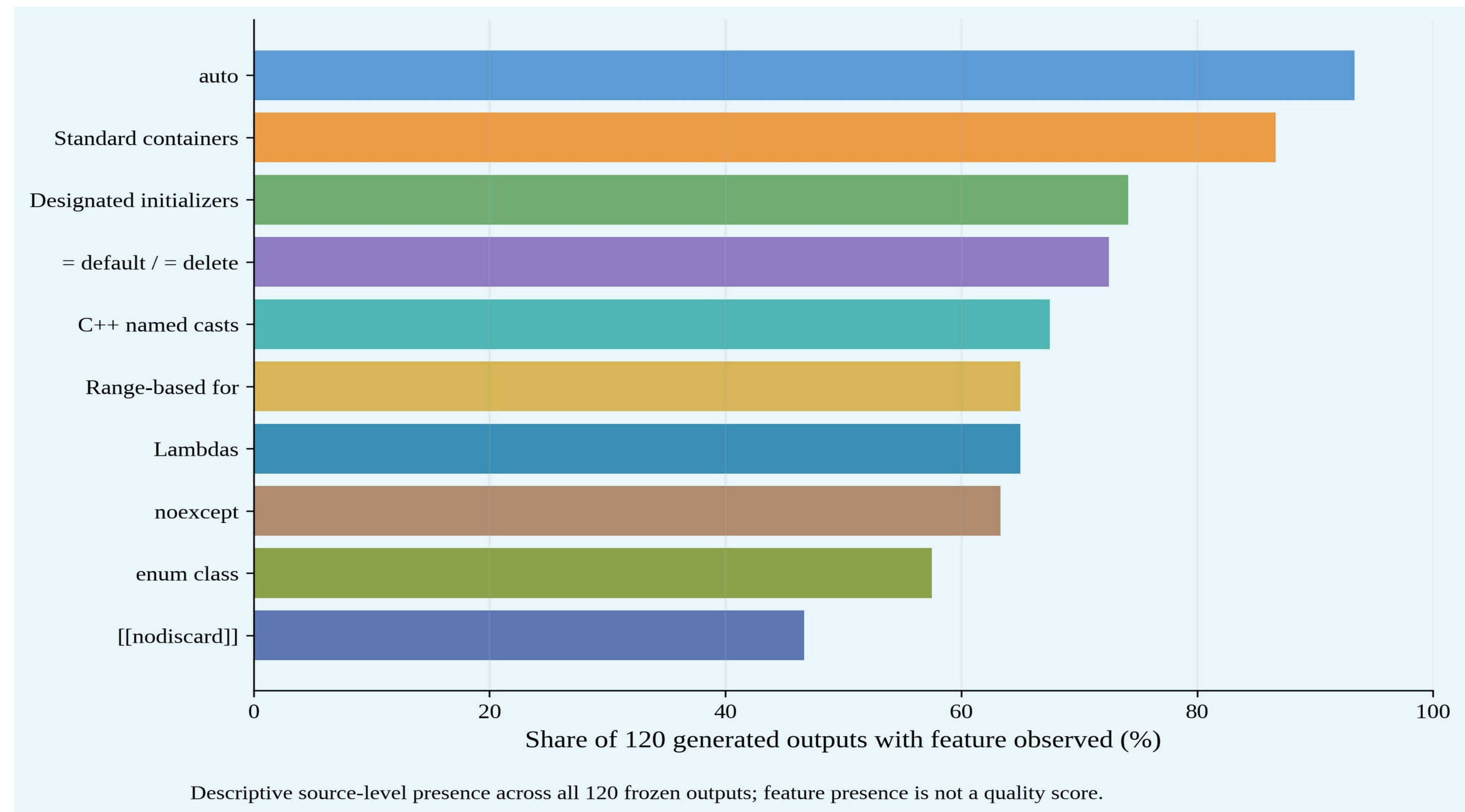
Figure 5. Most Frequently Observed Concrete Modern C++ Features
