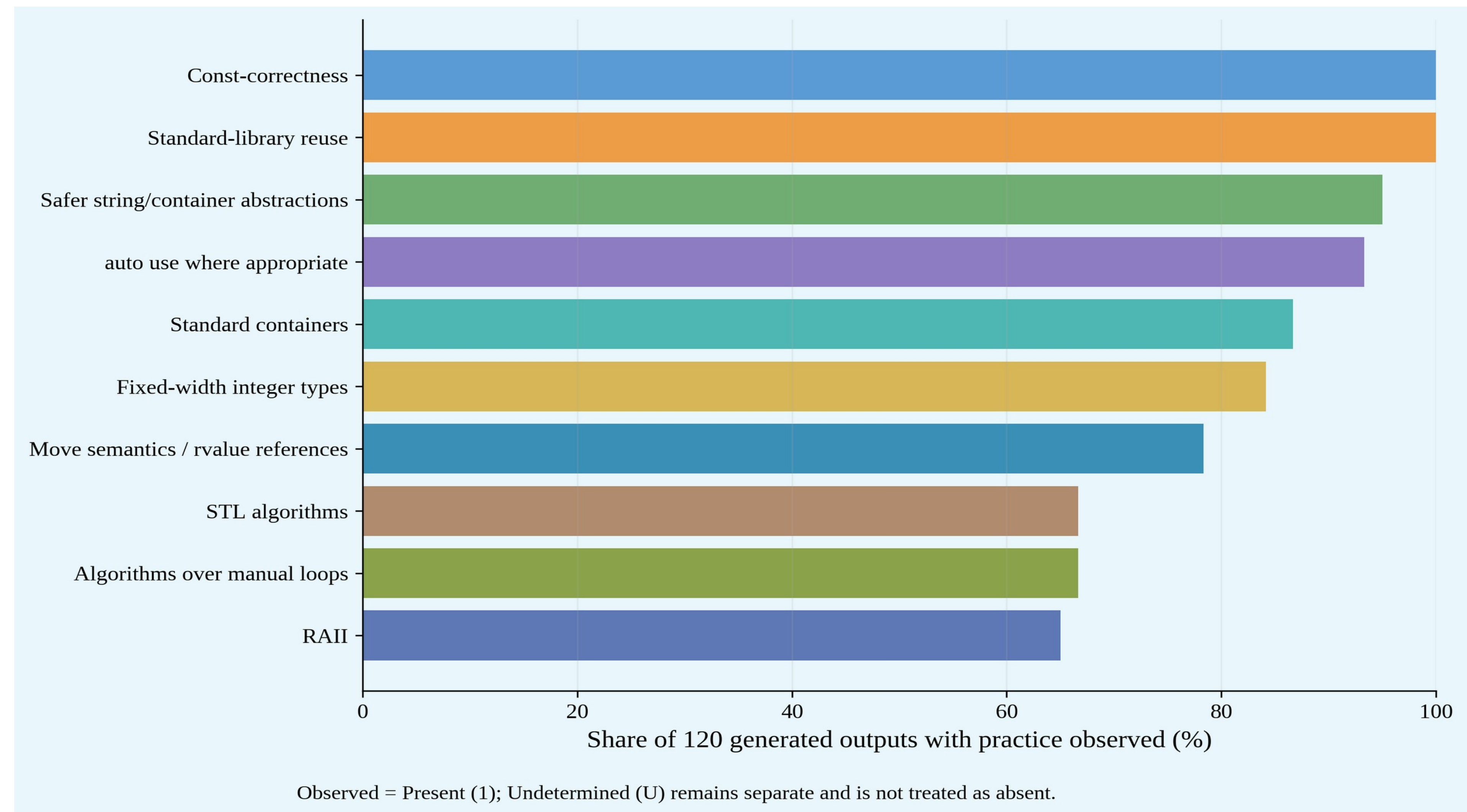
Figure 6. Most Frequently Observed Broader Modern C++ Practices
