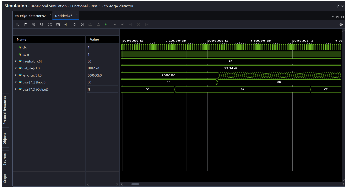
Figure 3: Simulation Waveform for Latency and Edge Response
