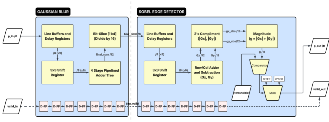
Figure 1: Hardware Architecture Block Diagram
