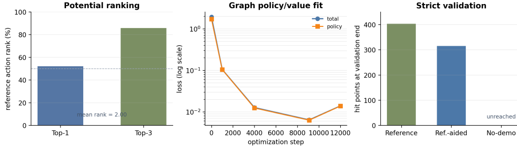
Figure 4: Summary of the main empirical signals. Left: the learned potential ranks the reference transition within the top three legal alternatives in most validated states. Middle: graph policy/value training reaches its best checkpoint before overfitting becomes visible. Right: deterministic replay separates reference validation, reference-aided closed-loop search, and the current no-demonstration archive search.
