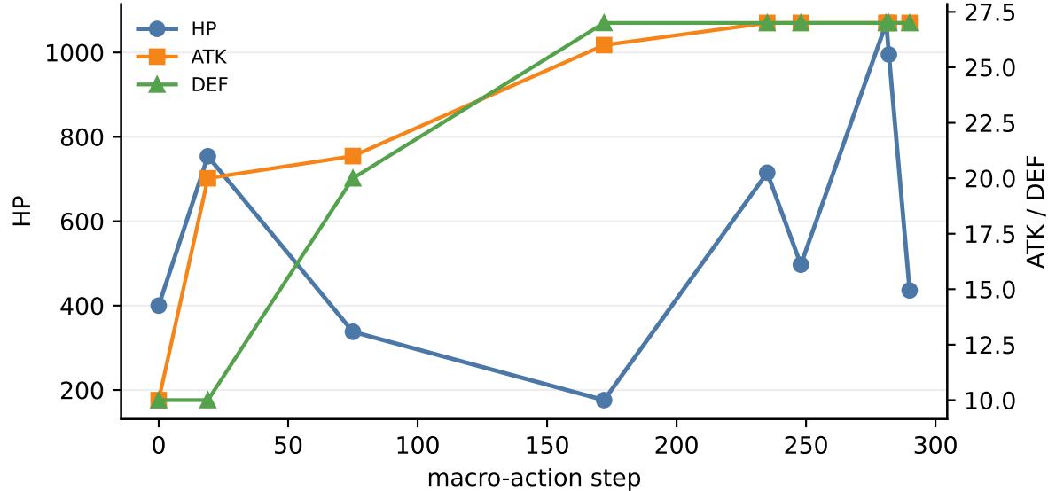
Checkpoint-level resources
