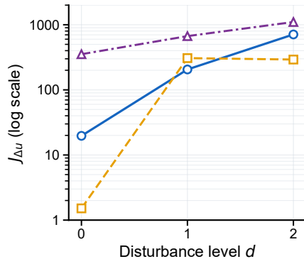
(c) Control smoothness cost
