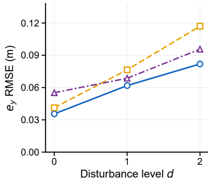
(a) Lateral-error RMSE
