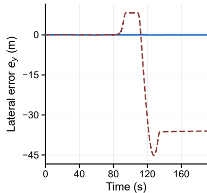
(c) Main-route lateral error
