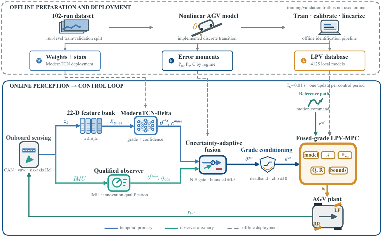
FIGURE 2. Overall slope-aware perception-and-control framework. The online loop separates the history-based primary branch from the bias-compensated six-axis Qualified observer branch. ModernTCN-delta supplies the primary grade and confidence; the Qualified observer contributes only an innovation-qualified, bounded correction with exact fallback to the ModernTCN estimate. The conditioned grade \hat{\theta}_k^{\text{ch}} synchronously updates the LPV scheduling vector, measured-disturbance channel, grade feedforward, weights, and constraints before the constrained MPC command is applied to the nonlinear AGV plant. Dashed gray arrows denote offline deployment of normalization statistics and network weights, fusion error moments, and the 4125-model LPV database.
