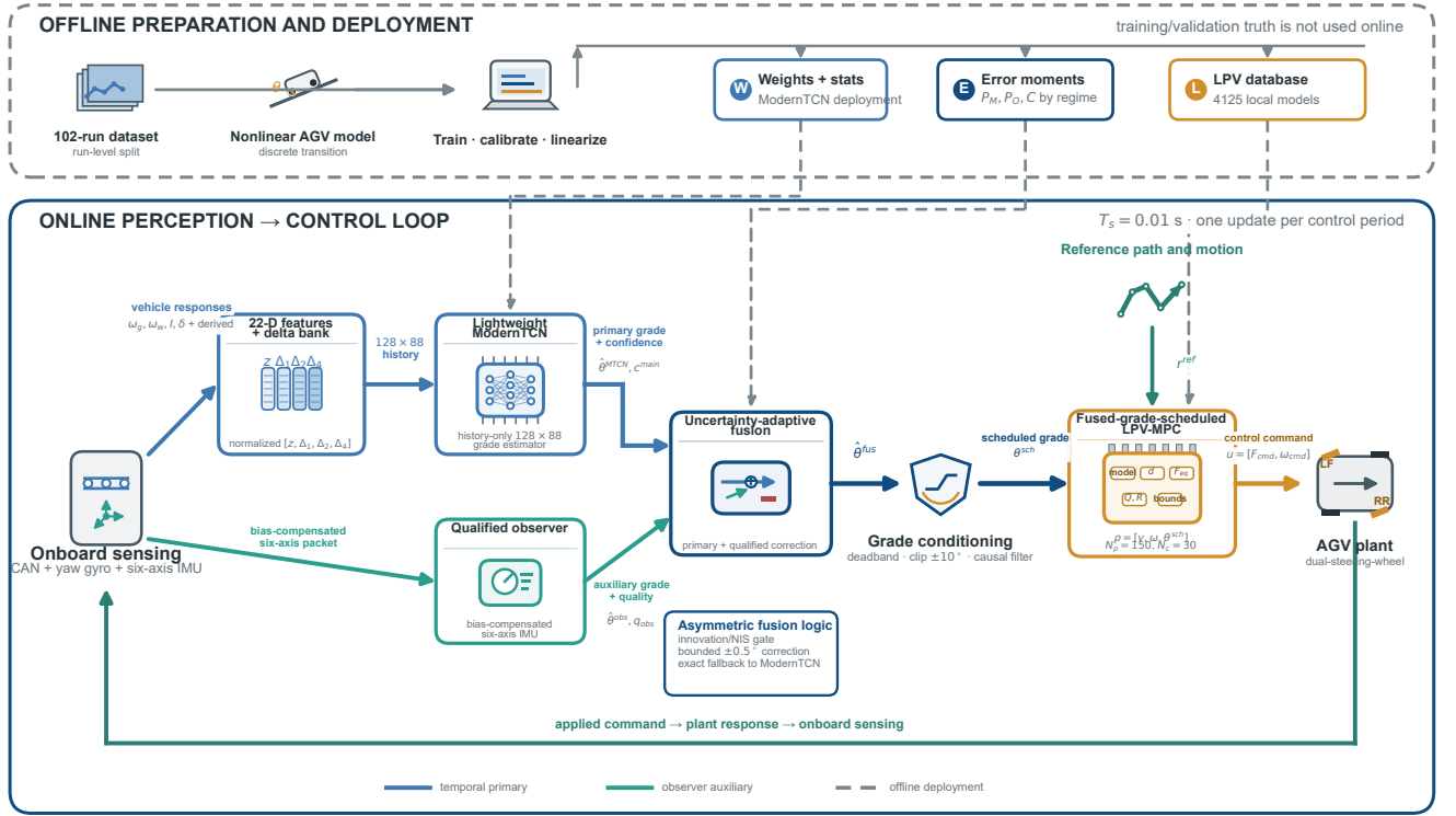
FIGURE 2. Overall slope-aware perception-and-control framework. The online loop separates the history-based primary branch from the bias-compensated six-axis Qualified observer branch. ModernTCN-delta supplies the primary grade and confidence; the Qualified observer contributes only an innovation-qualified, bounded correction with exact fallback to the ModernTCN estimate. The conditioned grade \hat{\theta}_k^{\text{sch}} synchronously updates the LPV scheduling vector, measured-disturbance channel, grade feedforward, weights, and constraints before the constrained MPC command is applied to the nonlinear AGV plant. Dashed gray arrows denote offline deployment of normalization statistics and network weights, fusion error moments, and the 4125-model LPV database.
